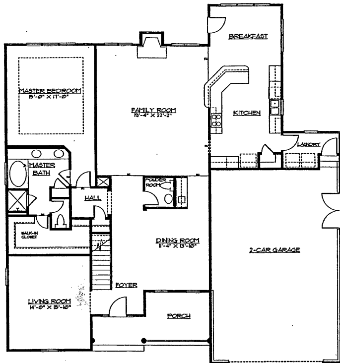
FIRST FLOOR PLAN 2-CAR GARAGE-FRONT LOAD
